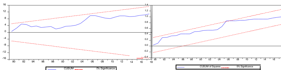
Figure 1: The plot of the Cumulative Sum (CUSUM). Source: Computed by Author's
